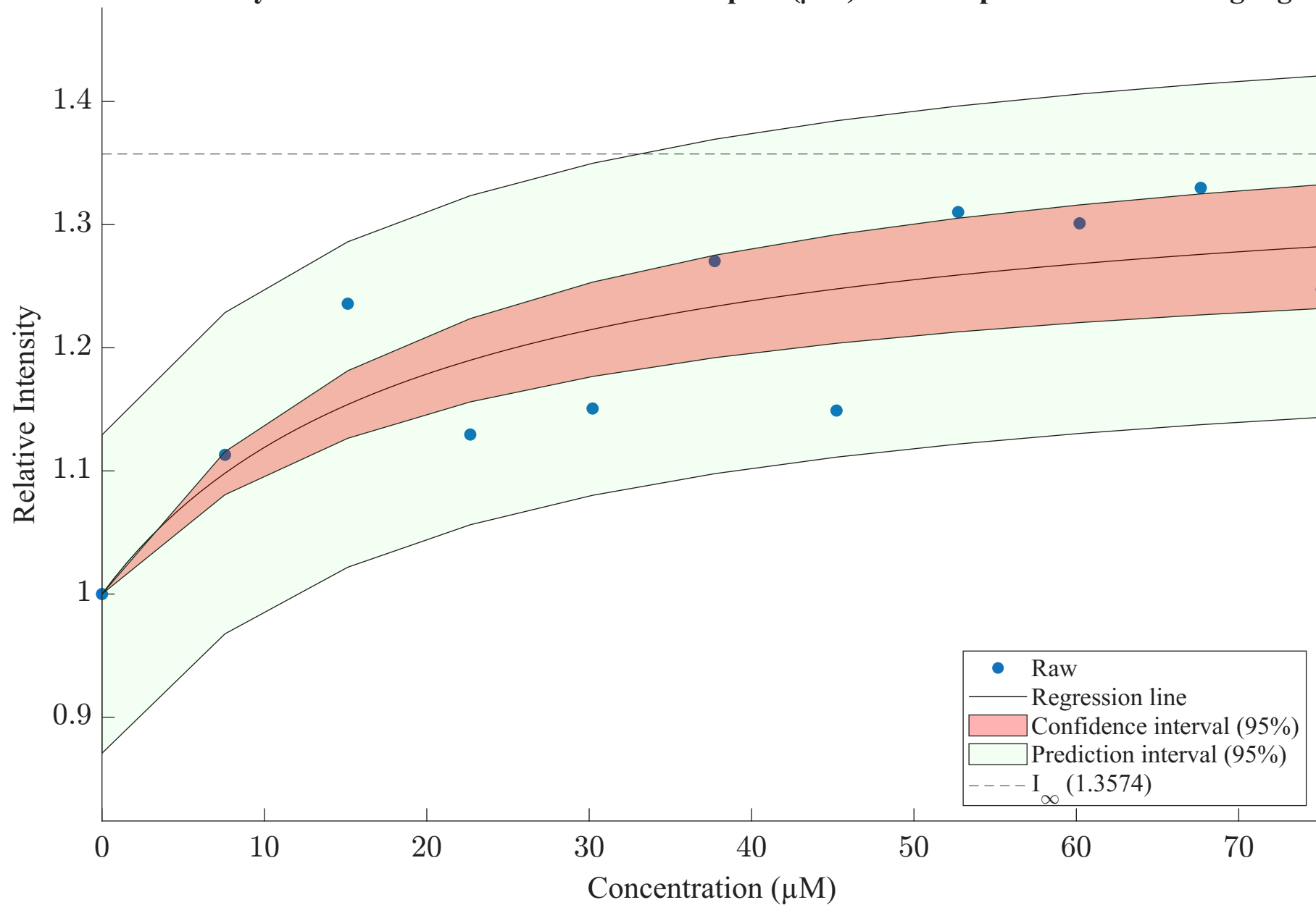
Relative intensity as a function of concentration of lipids ( \mu\text{M} ) for wt rep4 - Statistics fitting algorithm
